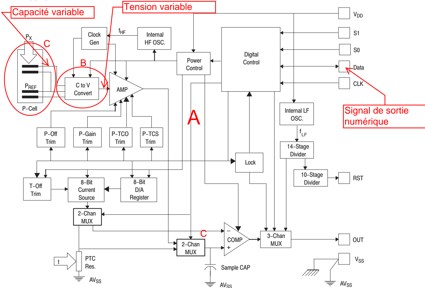
Figure 1. MPXY8020A Block Diagram
